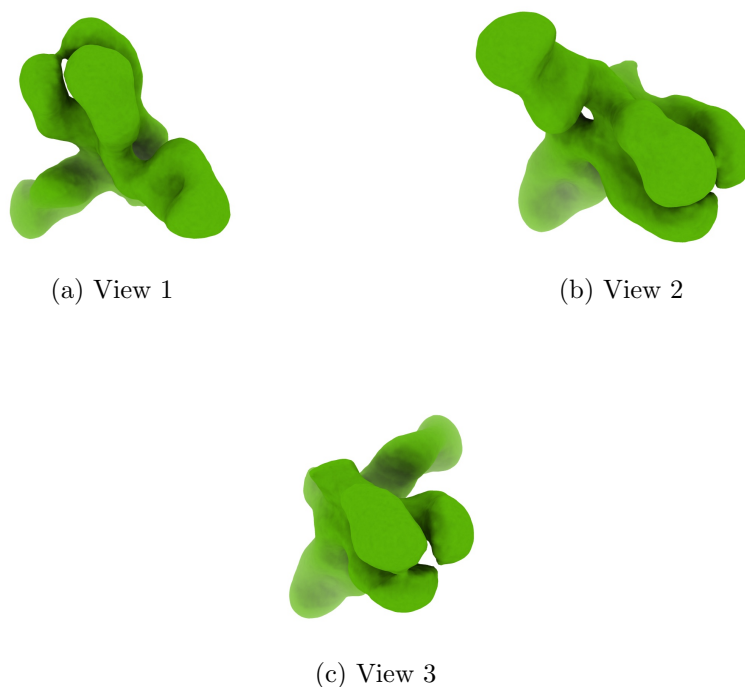
Figure 4: Isosurface at threshold=0.015300. Views generated by ChimeraX at a the following X, Y, Z angles: View 1 (0, -90, -90), View 2 (-90, 0, -90), View 3 (0, 0, 0).
