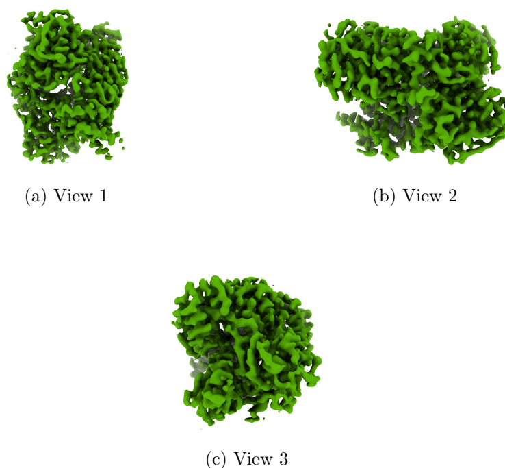
Figure 4: Isosurface at threshold=0.523000. Views generated by ChimeraX at a the following X, Y, Z angles: View 1 (0, -90, -90), View 2 (-90, 0, -90), View 3 (0, 0, 0).
