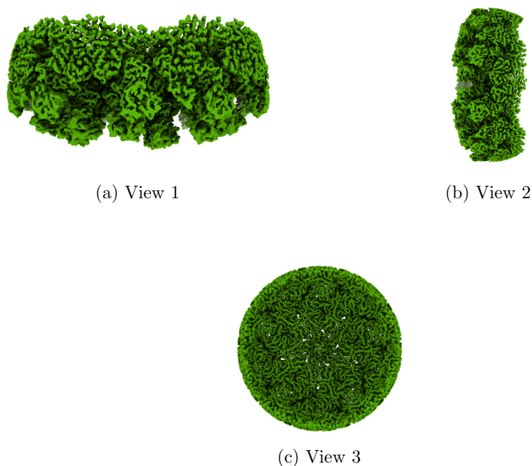
Figure 4: Isosurface at threshold=0.250000. Views generated by ChimeraX at a the following X, Y, Z angles: View 1 (0, -90, -90), View 2 (-90, 0, -90), View 3 (0, 0, 0).
