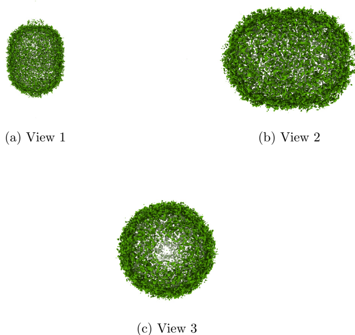
Figure 4: Isosurface at threshold=0.048600. Views generated by ChimeraX at a the following X, Y, Z angles: View 1 (0, -90, -90), View 2 (-90, 0, -90), View 3 (0, 0, 0).
