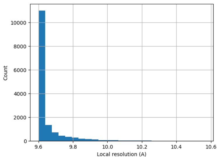
Figure 23: Histogram of the local resolution according to Resmap.
