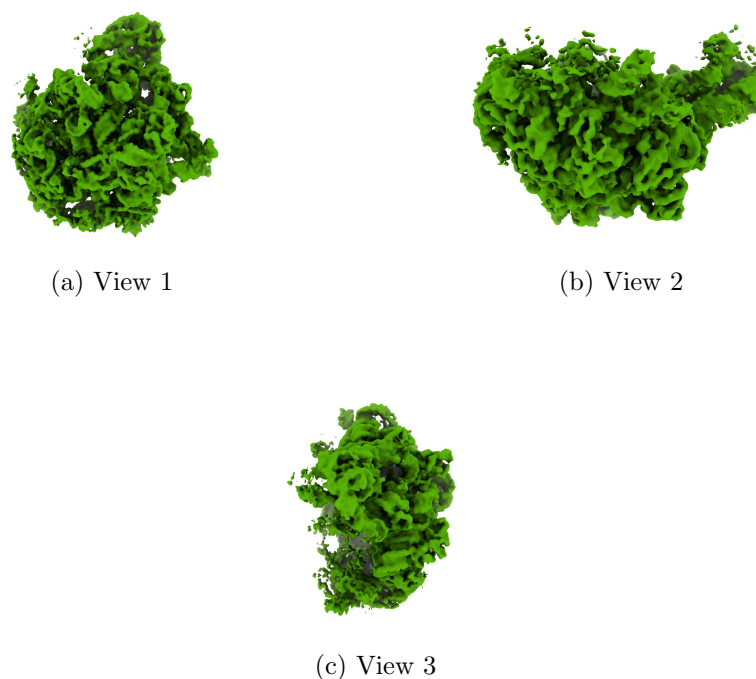
Figure 4: Isosurface at threshold=0.093000. Views generated by ChimeraX at a the following X, Y, Z angles: View 1 (0, -90, -90), View 2 (-90, 0, -90), View 3 (0, 0, 0).
