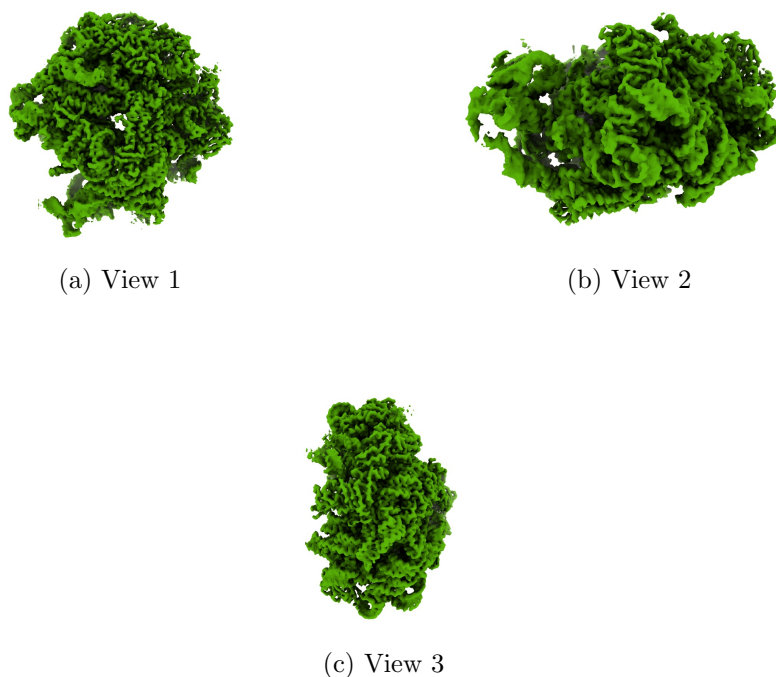
Figure 4: Isosurface at threshold=0.142000. Views generated by ChimeraX at a the following X, Y, Z angles: View 1 (0, -90, -90), View 2 (-90, 0, -90), View 3 (0, 0, 0).
