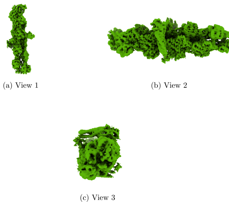
Figure 4: Isosurface at threshold=0.128000. Views generated by ChimeraX at a the following X, Y, Z angles: View 1 (0, -90, -90), View 2 (-90, 0, -90), View 3 (0, 0, 0).
