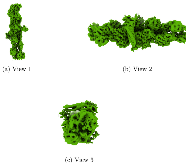
Figure 4: Isosurface at threshold=0.126000. Views generated by ChimeraX at a the following X, Y, Z angles: View 1 (0, -90, -90), View 2 (-90, 0, -90), View 3 (0, 0, 0).
