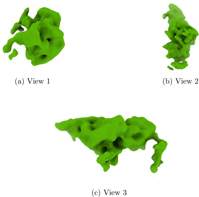
Figure 4: Isosurface at threshold=0.018600. Views generated by ChimeraX at a the following X, Y, Z angles: View 1 (0, -90, -90), View 2 (-90, 0, -90), View 3 (0, 0, 0).
