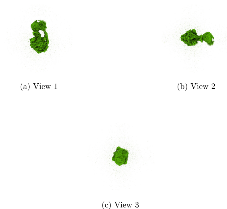
Figure 4: Isosurface at threshold=0.211000. Views generated by ChimeraX at a the following X, Y, Z angles: View 1 (0, -90, -90), View 2 (-90, 0, -90), View 3 (0, 0, 0).
