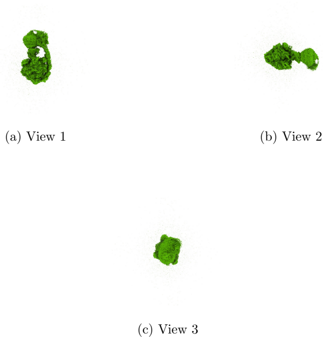
Figure 4: Isosurface at threshold=0.211000. Views generated by ChimeraX at a the following X, Y, Z angles: View 1 (0, -90, -90), View 2 (-90, 0, -90), View 3 (0, 0, 0).
