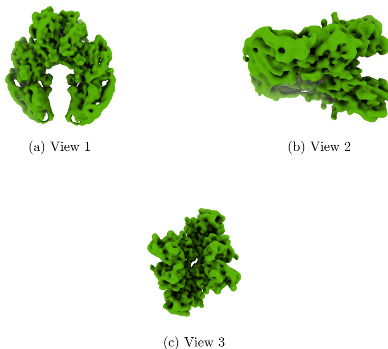
Figure 4: Isosurface at threshold=0.078500. Views generated by ChimeraX at a the following X, Y, Z angles: View 1 (0, -90, -90), View 2 (-90, 0, -90), View 3 (0, 0, 0).
