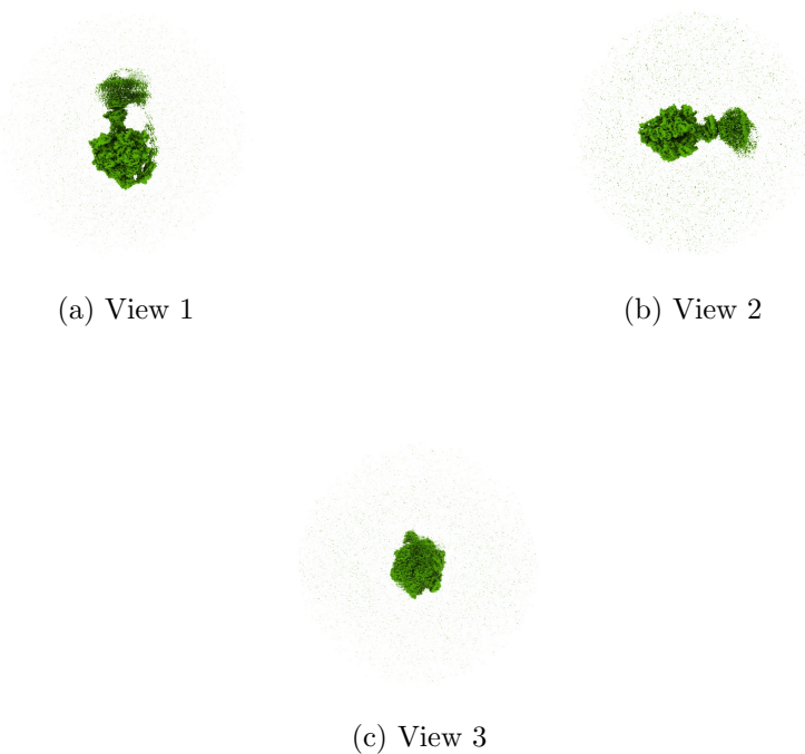
Figure 4: Isosurface at threshold=0.361000. Views generated by ChimeraX at a the following X, Y, Z angles: View 1 (0, -90, -90), View 2 (-90, 0, -90), View 3 (0, 0, 0).
