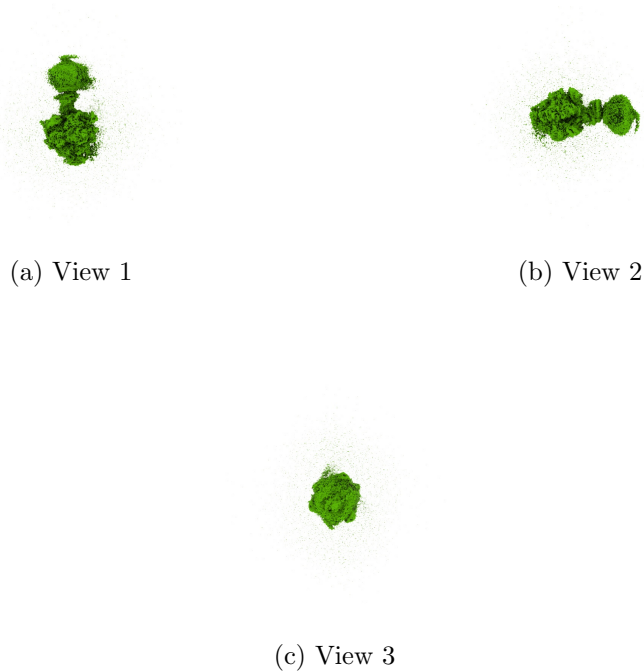
Figure 4: Isosurface at threshold=0.295000. Views generated by ChimeraX at a the following X, Y, Z angles: View 1 (0, -90, -90), View 2 (-90, 0, -90), View 3 (0, 0, 0).
