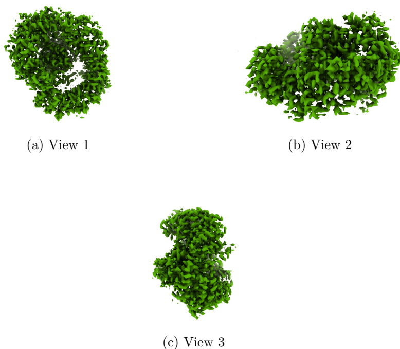
Figure 4: Isosurface at threshold=0.055000. Views generated by ChimeraX at a the following X, Y, Z angles: View 1 (0, -90, -90), View 2 (-90, 0, -90), View 3 (0, 0, 0).
