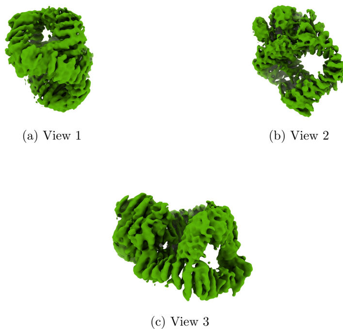
Figure 4: Isosurface at threshold=0.090600. Views generated by ChimeraX at a the following X, Y, Z angles: View 1 (0, -90, -90), View 2 (-90, 0, -90), View 3 (0, 0, 0).
