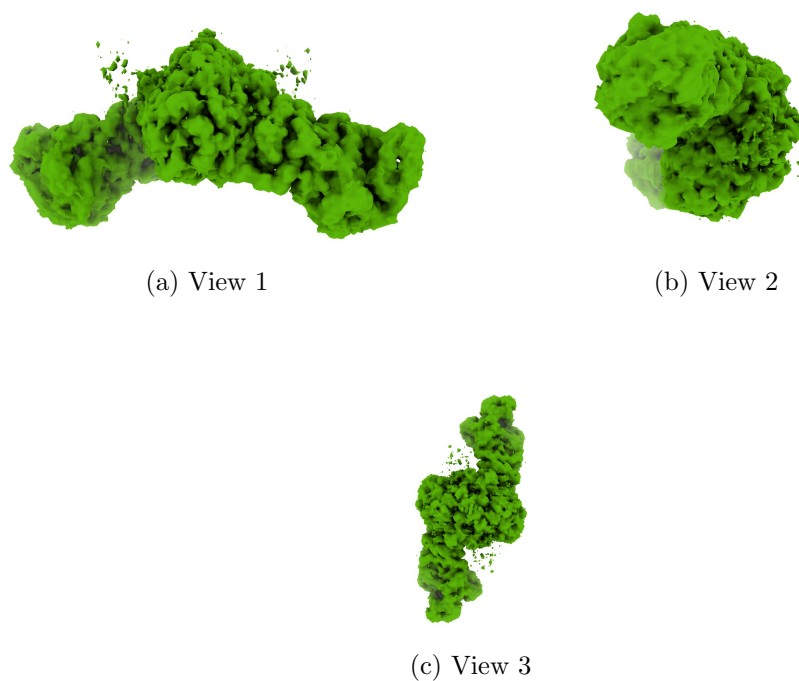
Figure 4: Isosurface at threshold=0.002070. Views generated by ChimeraX at a the following X, Y, Z angles: View 1 (0, -90, -90), View 2 (-90, 0, -90), View 3 (0, 0, 0).
