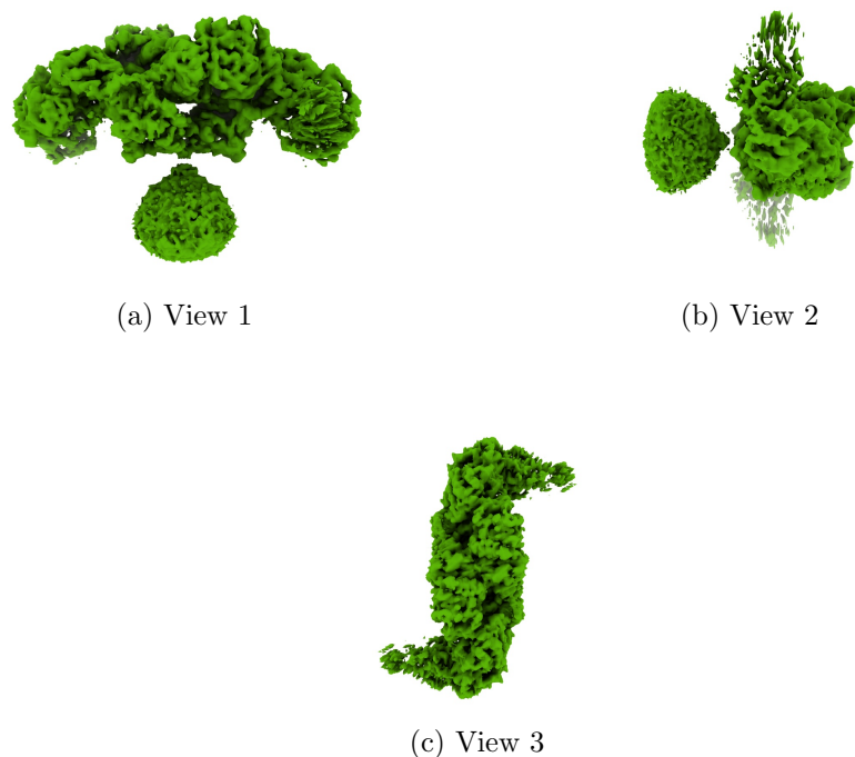
Figure 4: Isosurface at threshold=0.002640. Views generated by ChimeraX at a the following X, Y, Z angles: View 1 (0, -90, -90), View 2 (-90, 0, -90), View 3 (0, 0, 0).
