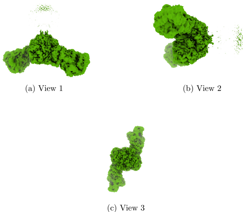
Figure 4: Isosurface at threshold=0.002220. Views generated by ChimeraX at a the following X, Y, Z angles: View 1 (0, -90, -90), View 2 (-90, 0, -90), View 3 (0, 0, 0).
