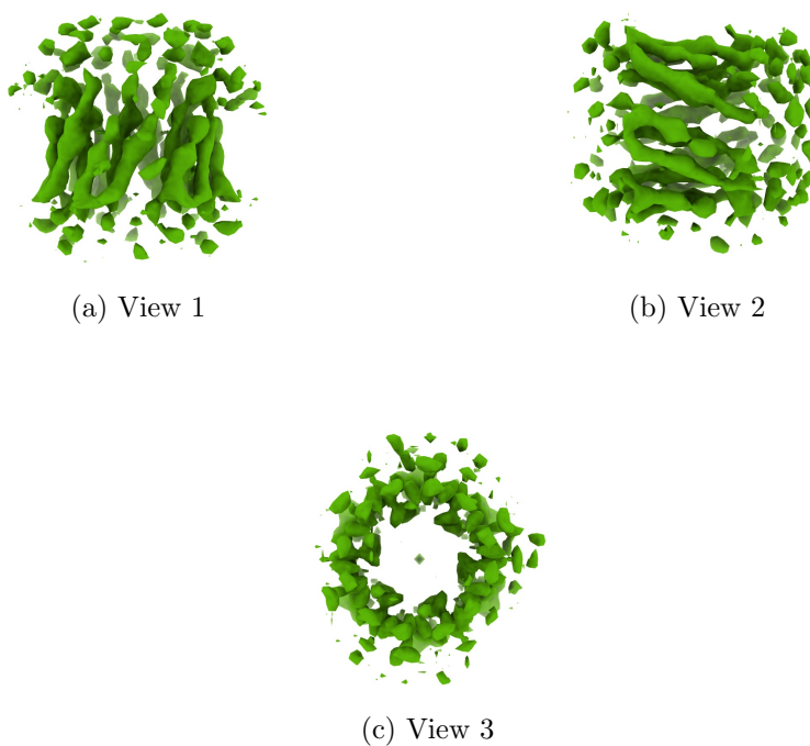
Figure 4: Isosurface at threshold=0.841000. Views generated by ChimeraX at a the following X, Y, Z angles: View 1 (0, -90, -90), View 2 (-90, 0, -90), View 3 (0, 0, 0).
