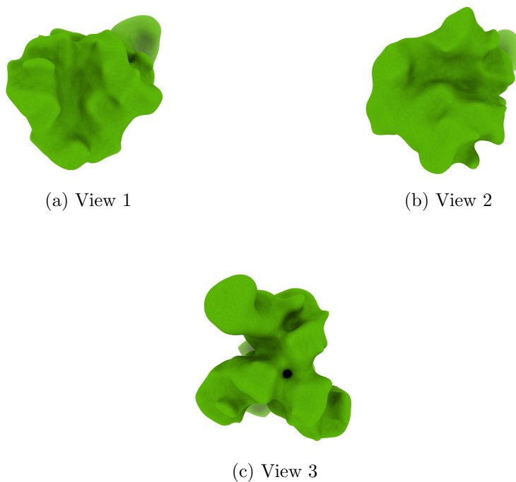
Figure 4: Isosurface at threshold=0.043100. Views generated by ChimeraX at a the following X, Y, Z angles: View 1 (0, -90, -90), View 2 (-90, 0, -90), View 3 (0, 0, 0).
