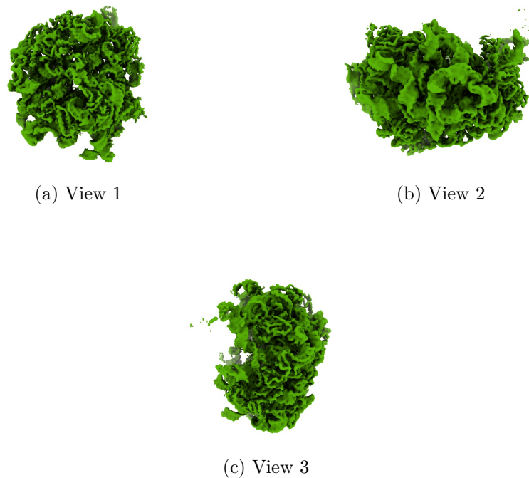
Figure 4: Isosurface at threshold=0.291000. Views generated by ChimeraX at a the following X, Y, Z angles: View 1 (0, -90, -90), View 2 (-90, 0, -90), View 3 (0, 0, 0).
