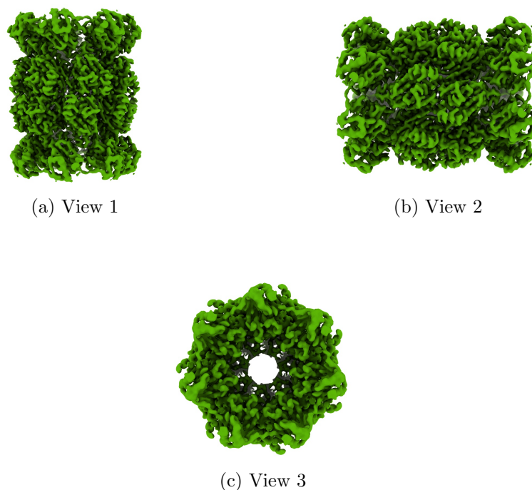
Figure 4: Isosurface at threshold=0.047300. Views generated by ChimeraX at a the following X, Y, Z angles: View 1 (0, -90, -90), View 2 (-90, 0, -90), View 3 (0, 0, 0).
