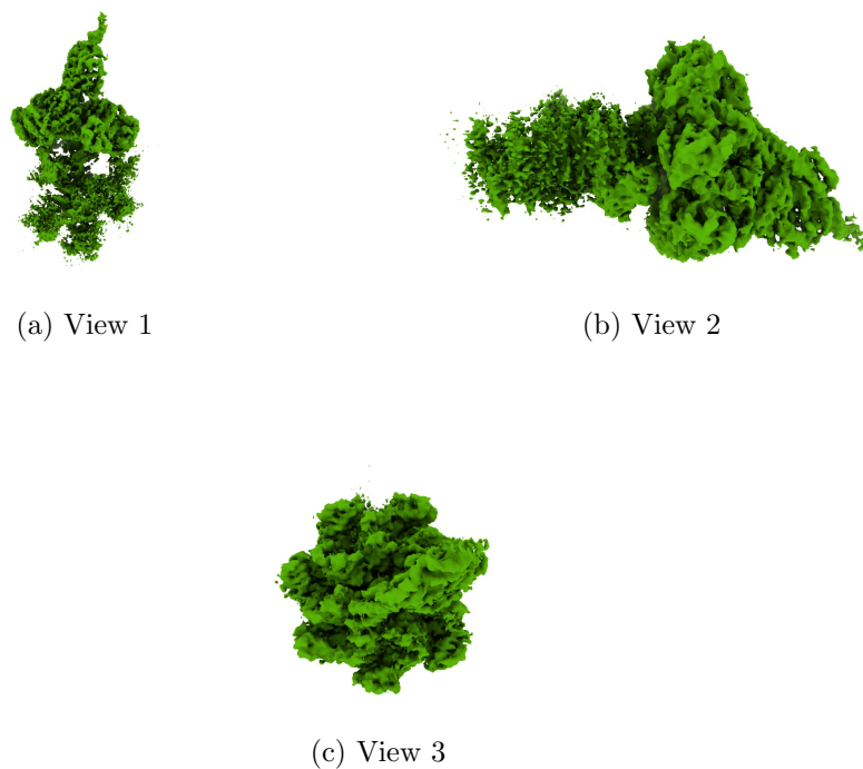
Figure 4: Isosurface at threshold=0.057600. Views generated by ChimeraX at a the following X, Y, Z angles: View 1 (0, -90, -90), View 2 (-90, 0, -90), View 3 (0, 0, 0).
