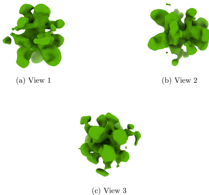
Figure 4: Isosurface at threshold=0.007730. Views generated by ChimeraX at a the following X, Y, Z angles: View 1 (0, -90, -90), View 2 (-90, 0, -90), View 3 (0, 0, 0).
