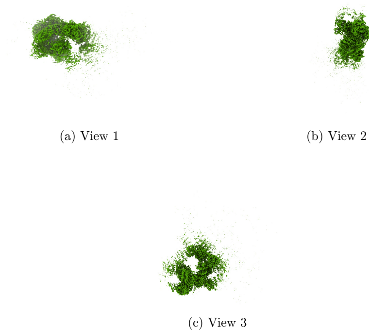
Figure 4: Isosurface at threshold=0.076800. Views generated by ChimeraX at a the following X, Y, Z angles: View 1 (0, -90, -90), View 2 (-90, 0, -90), View 3 (0, 0, 0).
