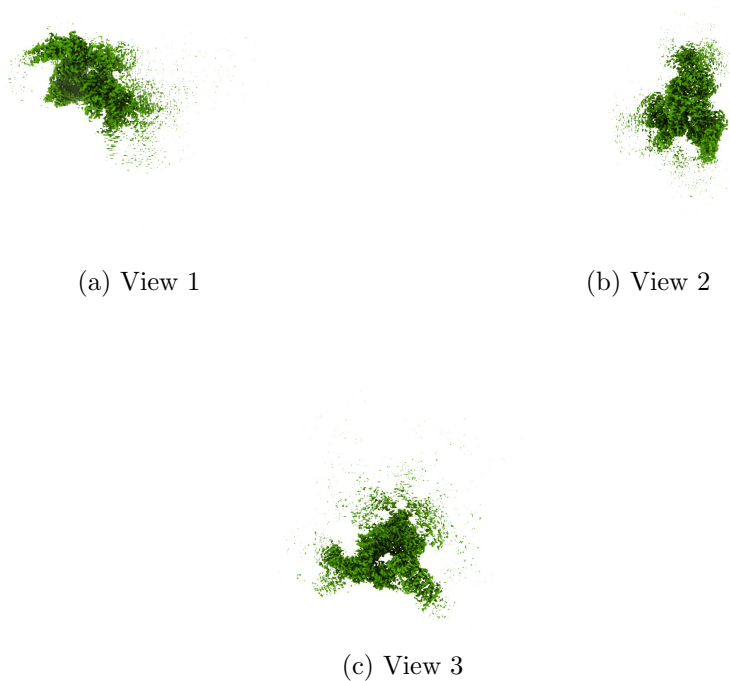
Figure 4: Isosurface at threshold=0.076800. Views generated by ChimeraX at a the following X, Y, Z angles: View 1 (0, -90, -90), View 2 (-90, 0, -90), View 3 (0, 0, 0).
