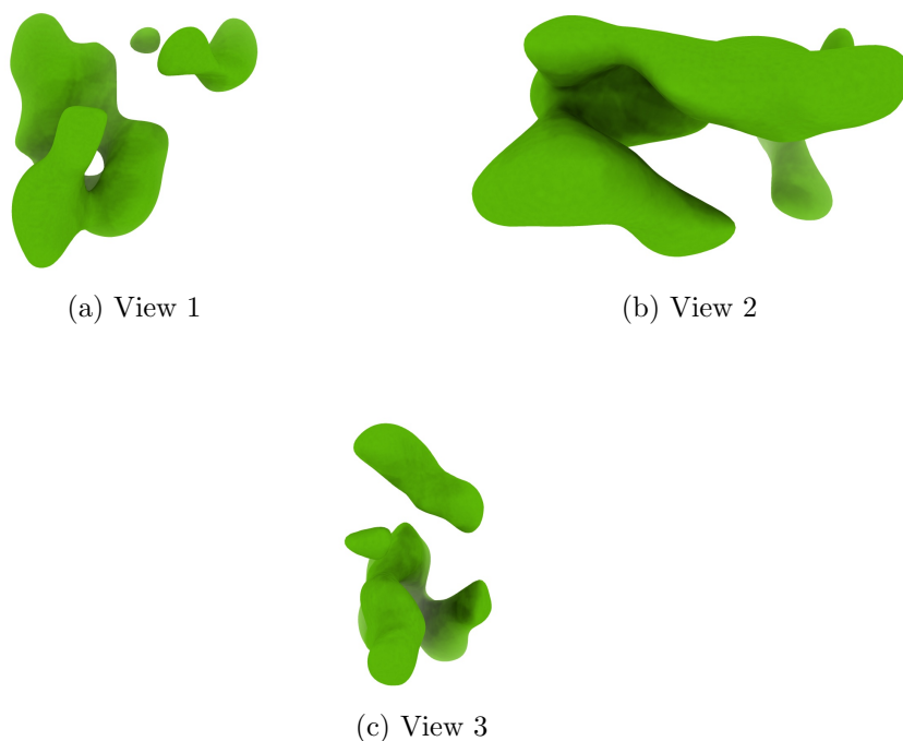
Figure 4: Isosurface at threshold=0.029400. Views generated by ChimeraX at a the following X, Y, Z angles: View 1 (0, -90, -90), View 2 (-90, 0, -90), View 3 (0, 0, 0).
