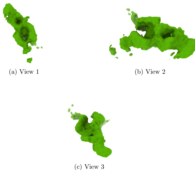
Figure 4: Isosurface at threshold=0.018700. Views generated by ChimeraX at a the following X, Y, Z angles: View 1 (0, -90, -90), View 2 (-90, 0, -90), View 3 (0, 0, 0).
