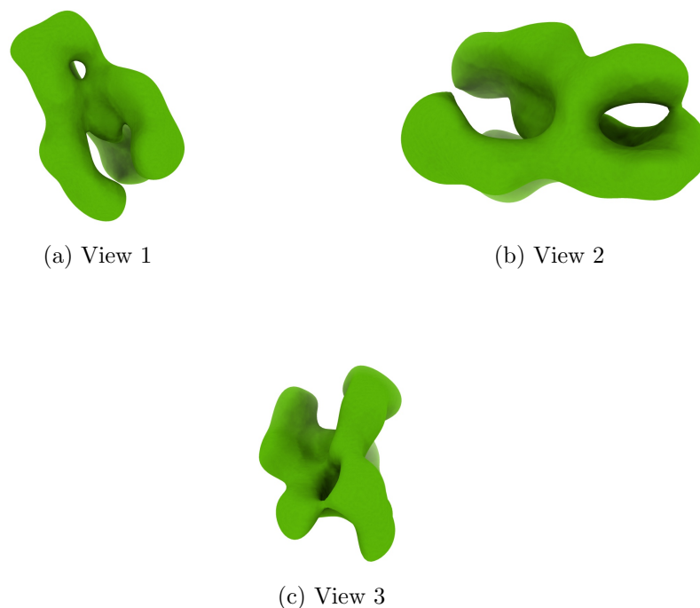
Figure 4: Isosurface at threshold=0.025800. Views generated by ChimeraX at a the following X, Y, Z angles: View 1 (0, -90, -90), View 2 (-90, 0, -90), View 3 (0, 0, 0).
