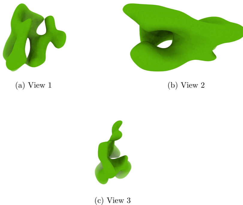
Figure 4: Isosurface at threshold=0.033100. Views generated by ChimeraX at a the following X, Y, Z angles: View 1 (0, -90, -90), View 2 (-90, 0, -90), View 3 (0, 0, 0).
