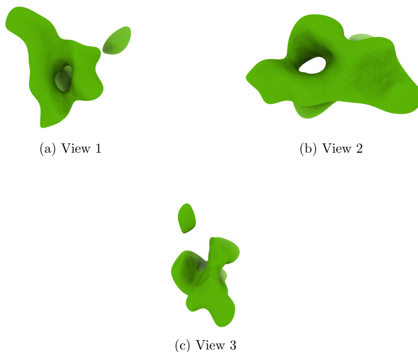
Figure 4: Isosurface at threshold=0.022200. Views generated by ChimeraX at a the following X, Y, Z angles: View 1 (0, -90, -90), View 2 (-90, 0, -90), View 3 (0, 0, 0).
