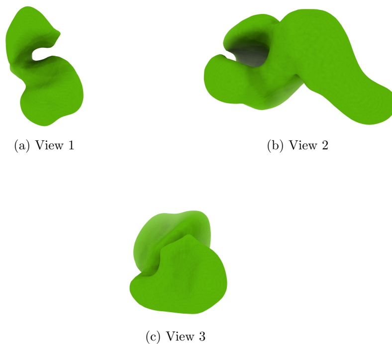
Figure 4: Isosurface at threshold=0.018100. Views generated by ChimeraX at a the following X, Y, Z angles: View 1 (0, -90, -90), View 2 (-90, 0, -90), View 3 (0, 0, 0).
