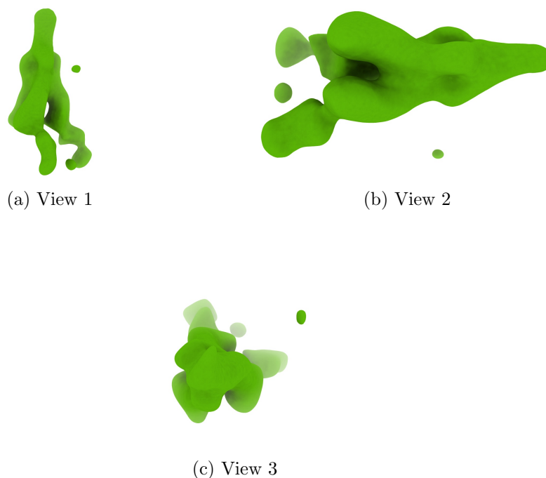
Figure 4: Isosurface at threshold=0.016700. Views generated by ChimeraX at a the following X, Y, Z angles: View 1 (0, -90, -90), View 2 (-90, 0, -90), View 3 (0, 0, 0).
