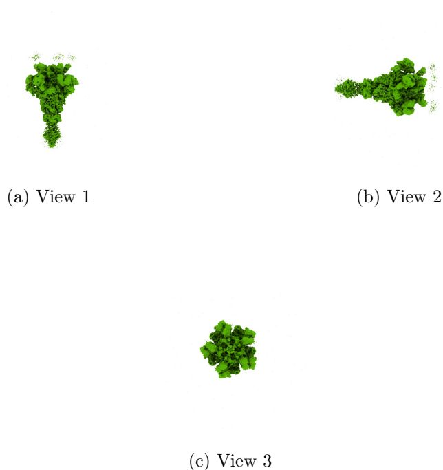
Figure 4: Isosurface at threshold=0.310000. Views generated by ChimeraX at a the following X, Y, Z angles: View 1 (0, -90, -90), View 2 (-90, 0, -90), View 3 (0, 0, 0).
