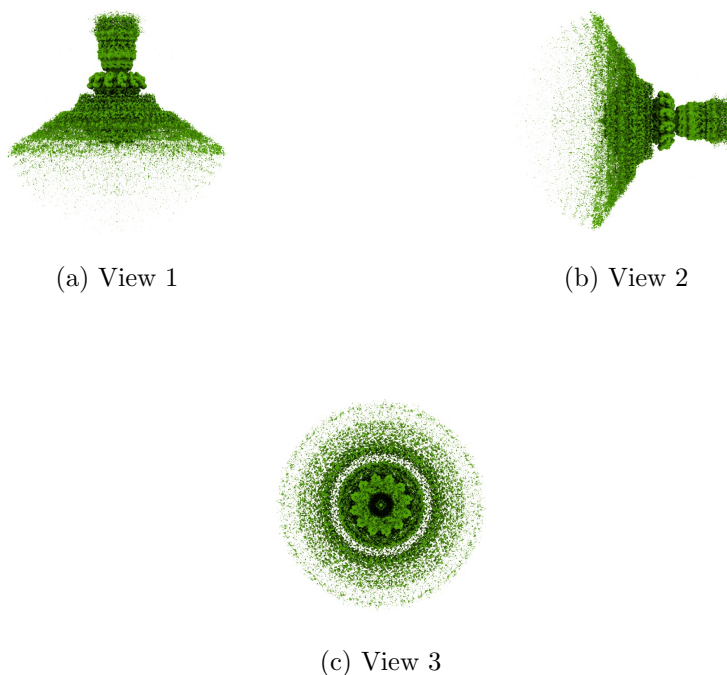
Figure 4: Isosurface at threshold=0.434000. Views generated by ChimeraX at a the following X, Y, Z angles: View 1 (0, -90, -90), View 2 (-90, 0, -90), View 3 (0, 0, 0).
