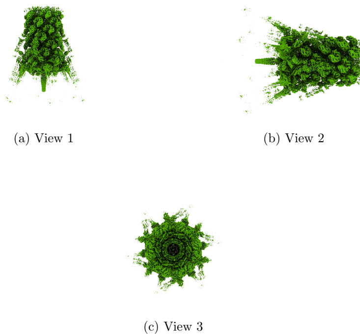
Figure 4: Isosurface at threshold=0.983000. Views generated by ChimeraX at a the following X, Y, Z angles: View 1 (0, -90, -90), View 2 (-90, 0, -90), View 3 (0, 0, 0).
