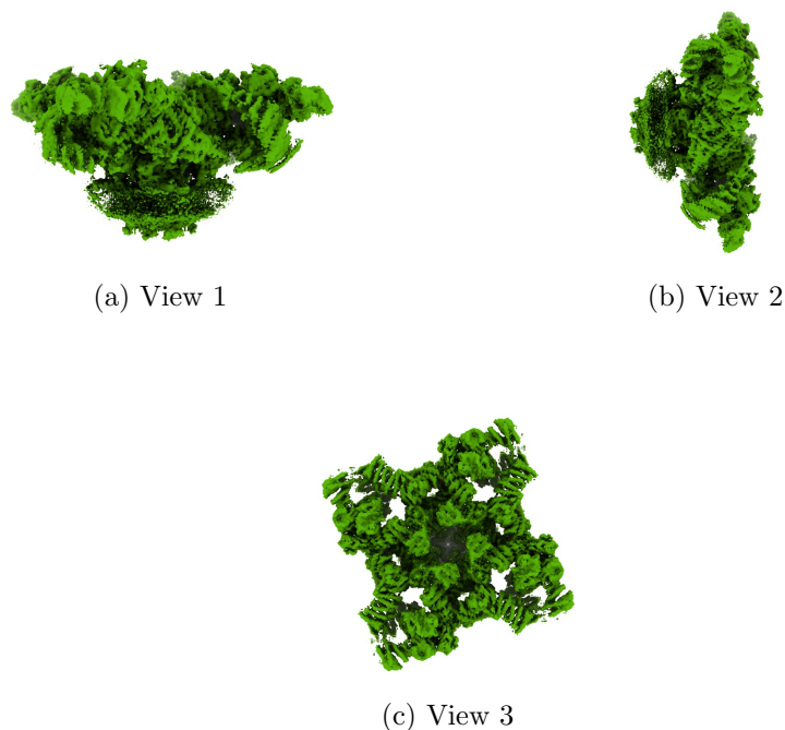
Figure 4: Isosurface at threshold=0.329000. Views generated by ChimeraX at a the following X, Y, Z angles: View 1 (0, -90, -90), View 2 (-90, 0, -90), View 3 (0, 0, 0).
