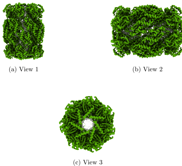
Figure 4: Isosurface at threshold=37.100000. Views generated by ChimeraX at a the following X, Y, Z angles: View 1 (0, -90, -90), View 2 (-90, 0, -90), View 3 (0, 0, 0).
