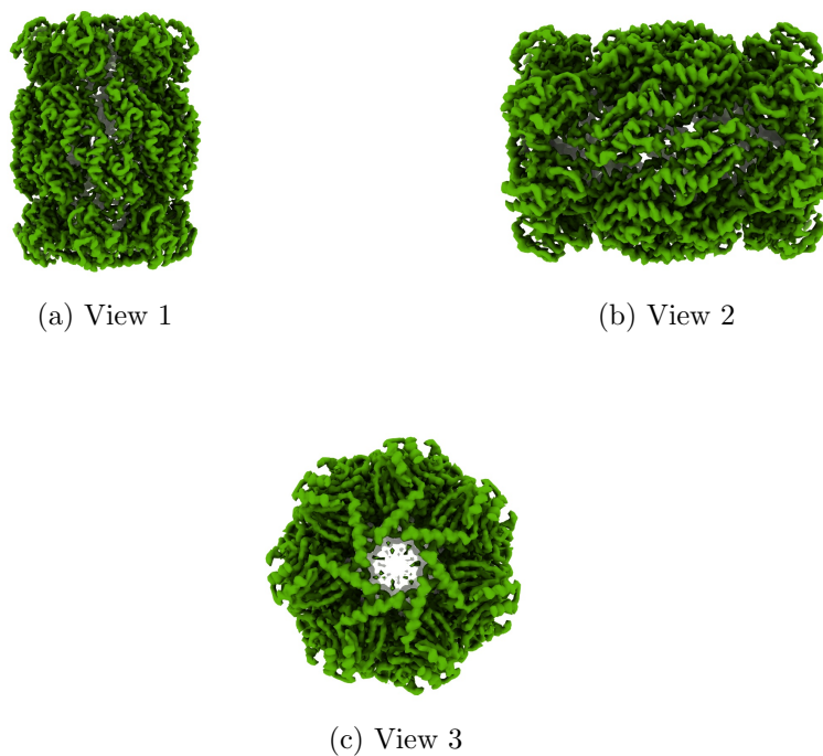
Figure 4: Isosurface at threshold=34.600000. Views generated by ChimeraX at a the following X, Y, Z angles: View 1 (0, -90, -90), View 2 (-90, 0, -90), View 3 (0, 0, 0).
