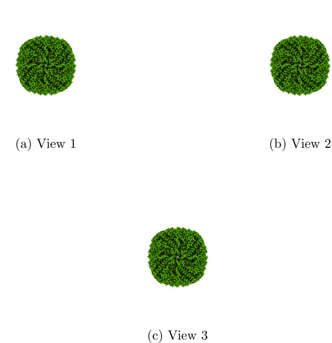
Figure 4: Isosurface at threshold=0.023000. Views generated by ChimeraX at a the following X, Y, Z angles: View 1 (0, -90, -90), View 2 (-90, 0, -90), View 3 (0, 0, 0).
