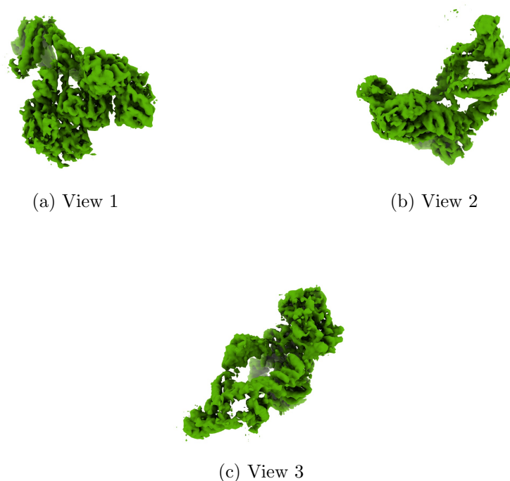
Figure 4: Isosurface at threshold=0.045900. Views generated by ChimeraX at a the following X, Y, Z angles: View 1 (0, -90, -90), View 2 (-90, 0, -90), View 3 (0, 0, 0).
