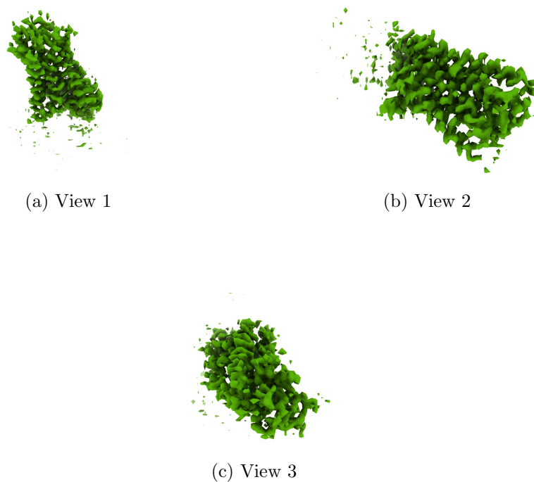
Figure 4: Isosurface at threshold=0.587000. Views generated by ChimeraX at a the following X, Y, Z angles: View 1 (0, -90, -90), View 2 (-90, 0, -90), View 3 (0, 0, 0).
