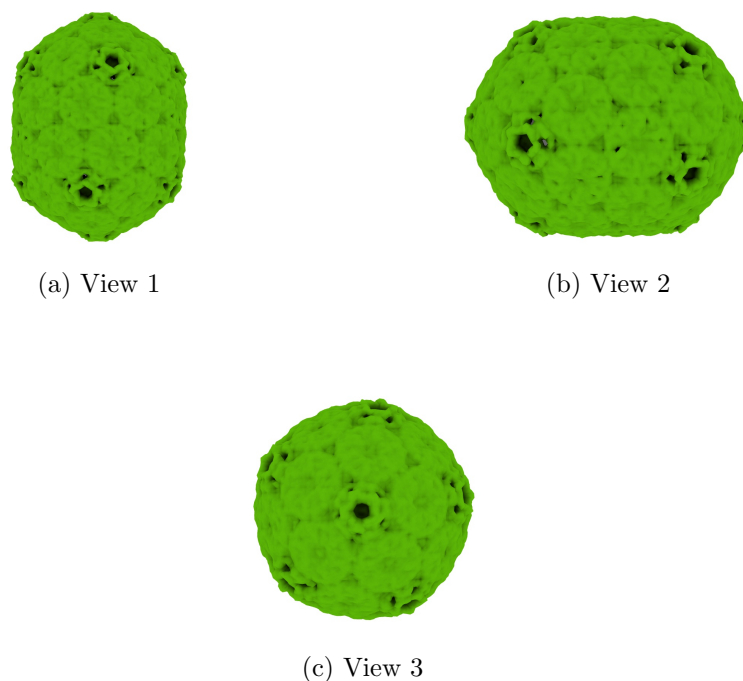
Figure 4: Isosurface at threshold=0.140000. Views generated by ChimeraX at a the following X, Y, Z angles: View 1 (0, -90, -90), View 2 (-90, 0, -90), View 3 (0, 0, 0).
