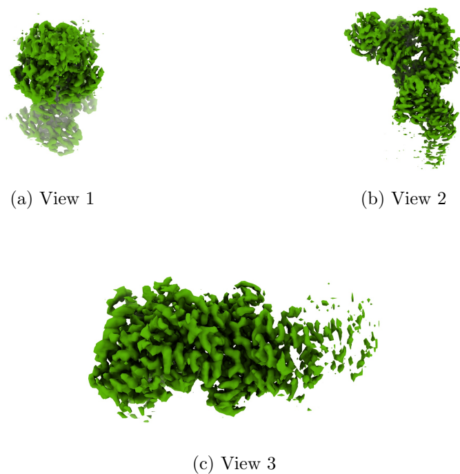
Figure 4: Isosurface at threshold=0.350000. Views generated by ChimeraX at a the following X, Y, Z angles: View 1 (0, -90, -90), View 2 (-90, 0, -90), View 3 (0, 0, 0).
