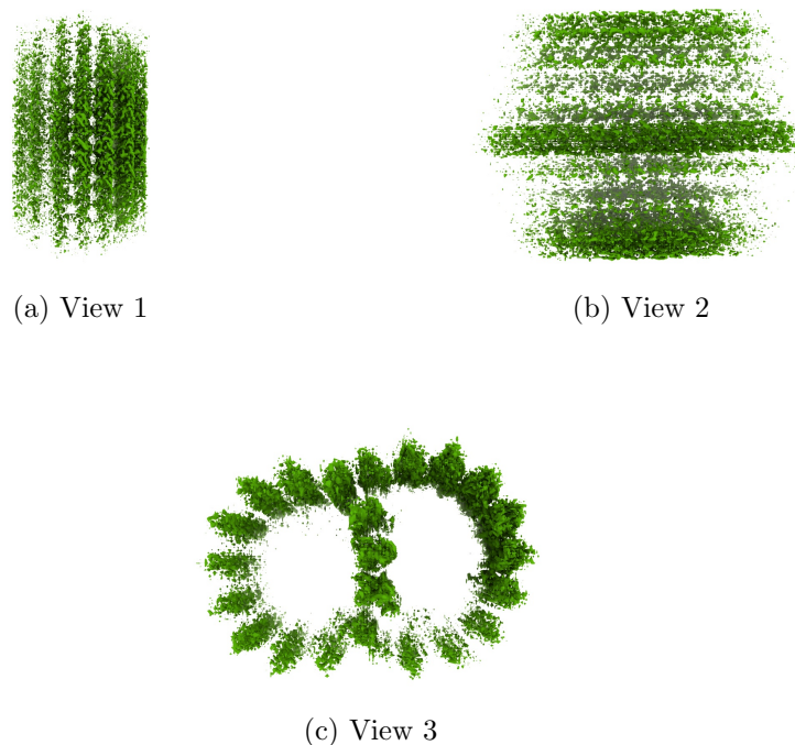
Figure 4: Isosurface at threshold=0.083700. Views generated by ChimeraX at a the following X, Y, Z angles: View 1 (0, -90, -90), View 2 (-90, 0, -90), View 3 (0, 0, 0).
