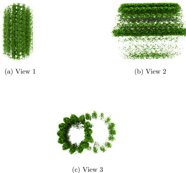
Figure 4: Isosurface at threshold=0.084400. Views generated by ChimeraX at a the following X, Y, Z angles: View 1 (0, -90, -90), View 2 (-90, 0, -90), View 3 (0, 0, 0).
