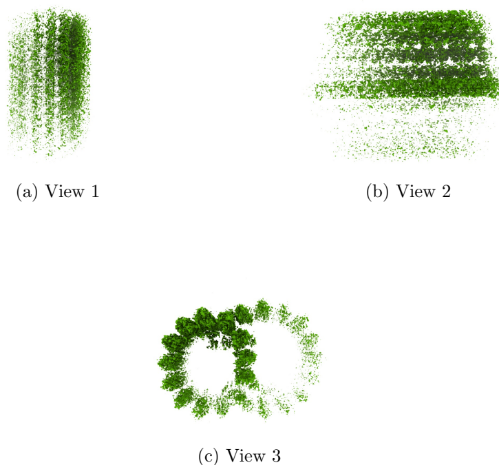
Figure 4: Isosurface at threshold=0.094700. Views generated by ChimeraX at a the following X, Y, Z angles: View 1 (0, -90, -90), View 2 (-90, 0, -90), View 3 (0, 0, 0).
