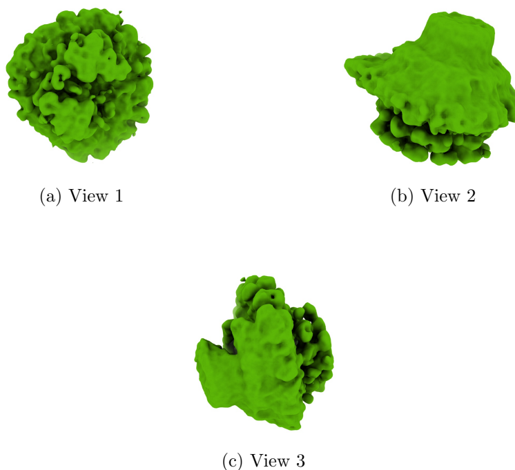
Figure 4: Isosurface at threshold=0.040800. Views generated by ChimeraX at a the following X, Y, Z angles: View 1 (0, -90, -90), View 2 (-90, 0, -90), View 3 (0, 0, 0).
